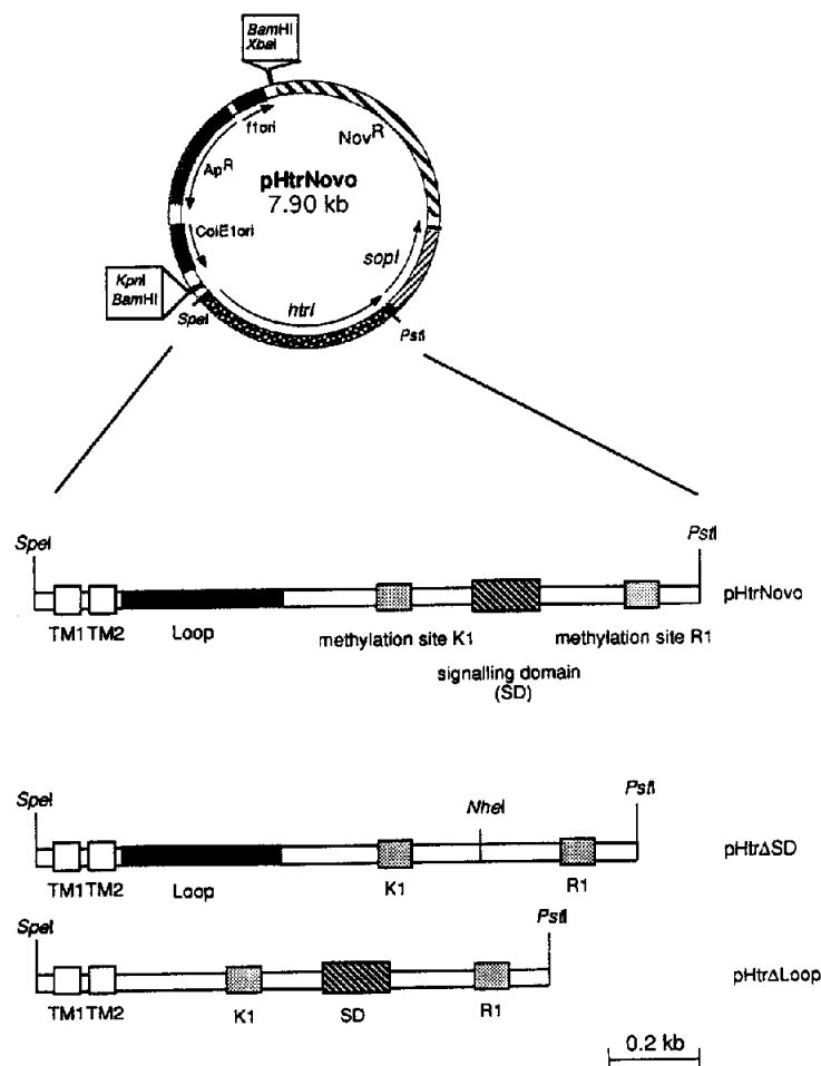
Fig. 2. The htrI mutagenesis vector pHtrNovo and its derivatives pHtrΔSD and pHtrΔLoop. The putative functional domains of the htrI gene, the two transmembrane helices (TM1, TM2), the cytoplasmic loop (loop), the methylation sites (K1 and R1) and the signalling domain (SD), are indicated in each of the constructs.
